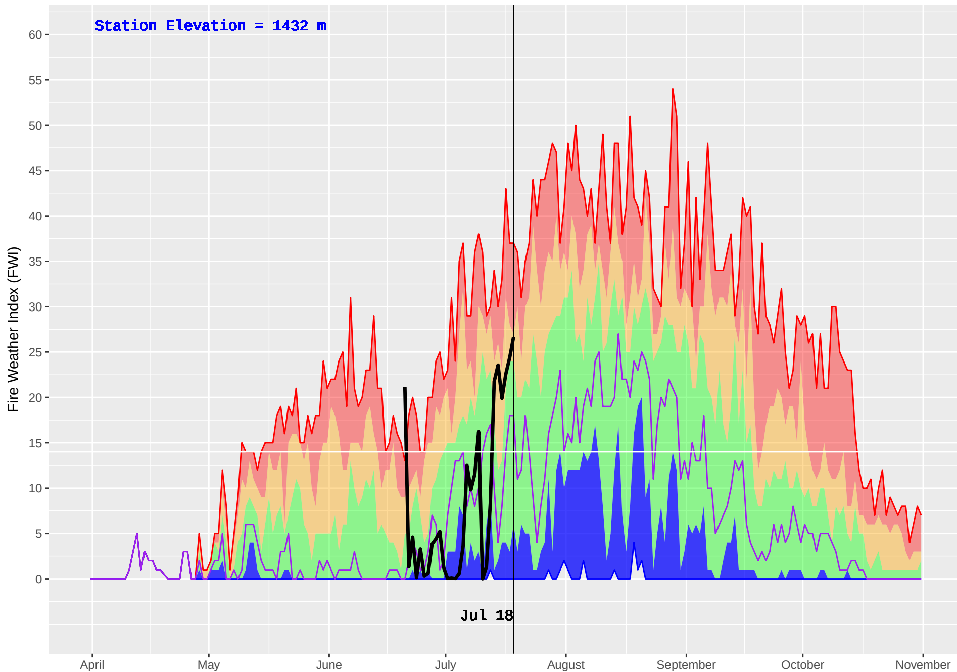
OCTOPUS CREEK (396) : Historical (2000–2016) and Current (2018) Daily Fire Weather Index (FWI)
