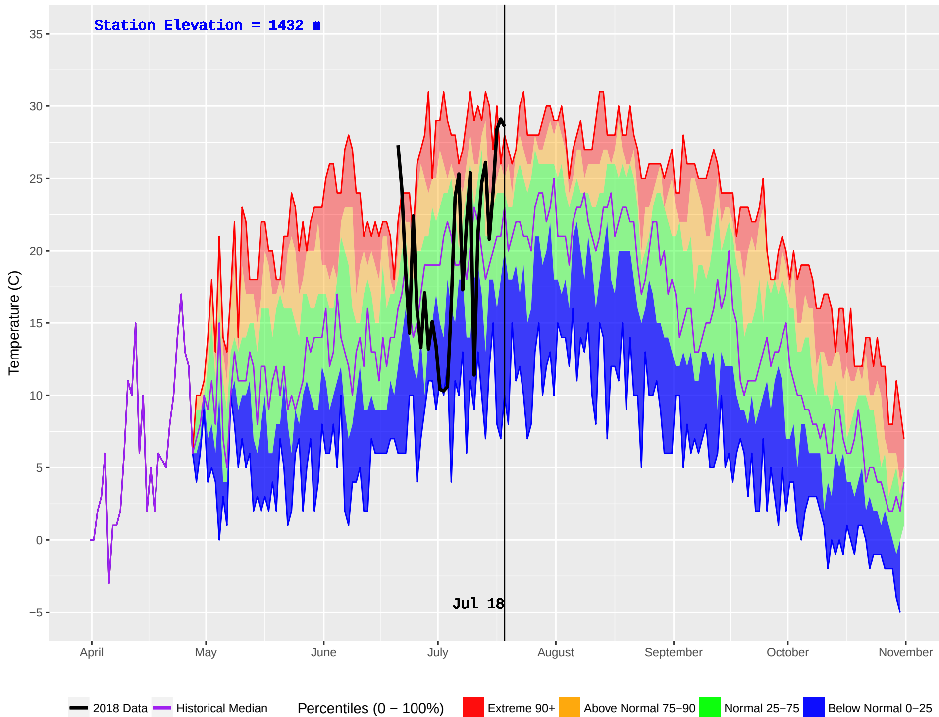
OCTOPUS CREEK (396) : Historical (2000–2016) and Current (2018) Daily Temperature
