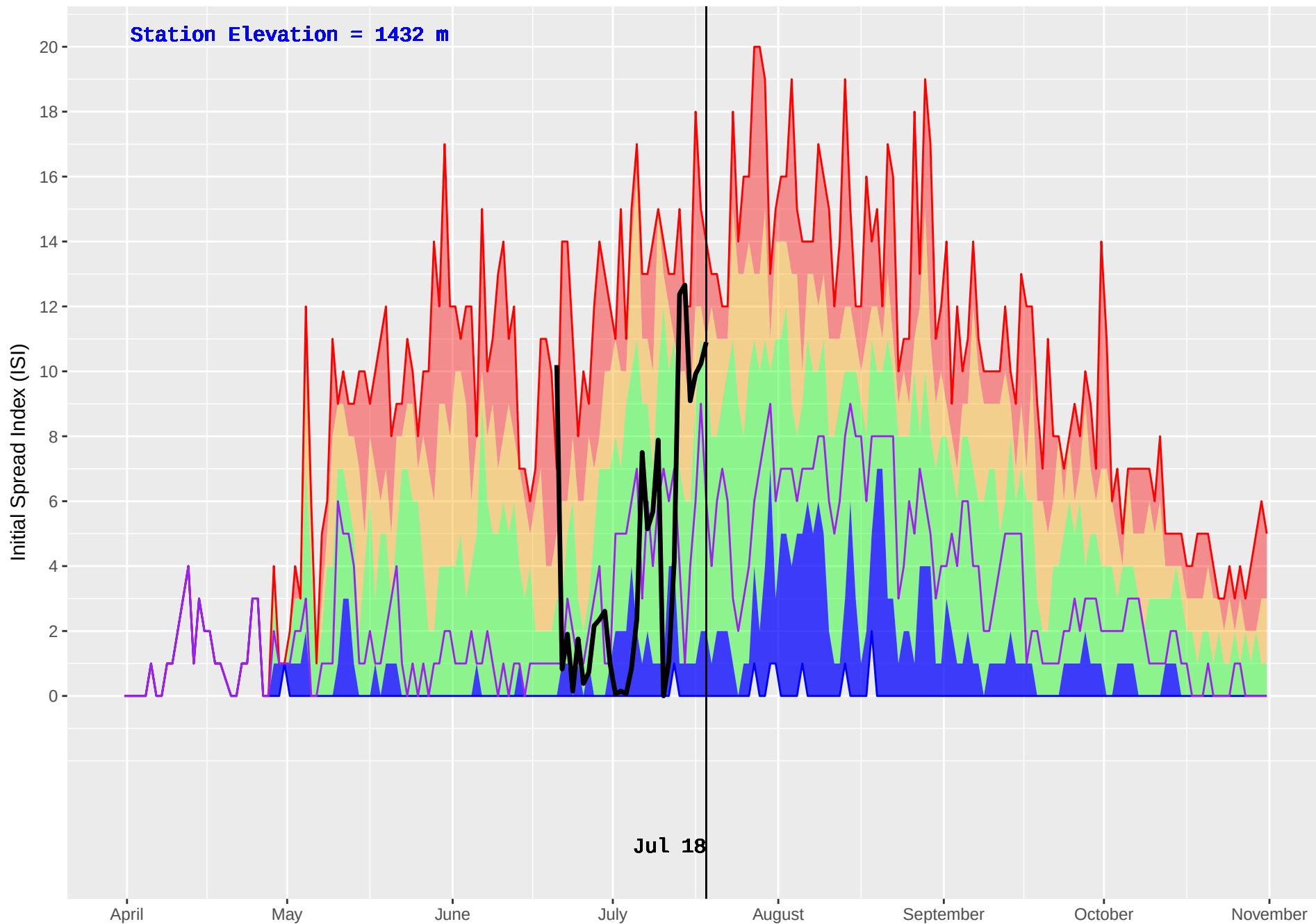
OCTOPUS CREEK (396) : Historical (2000–2016) and Current (2018) Daily Initial Spread Index (ISI)
